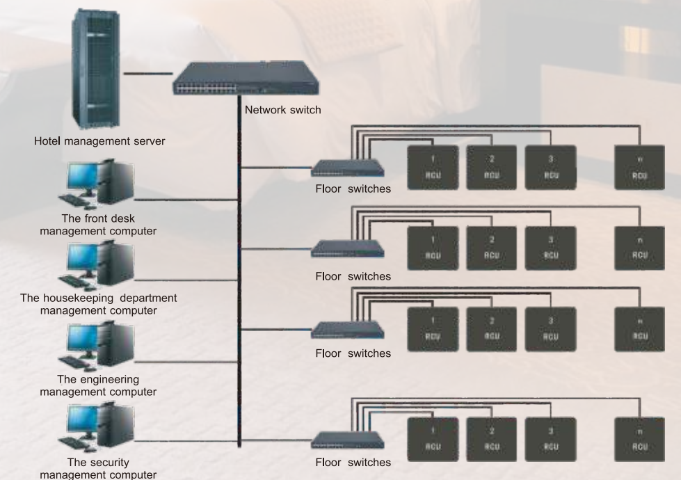
Network diagram
